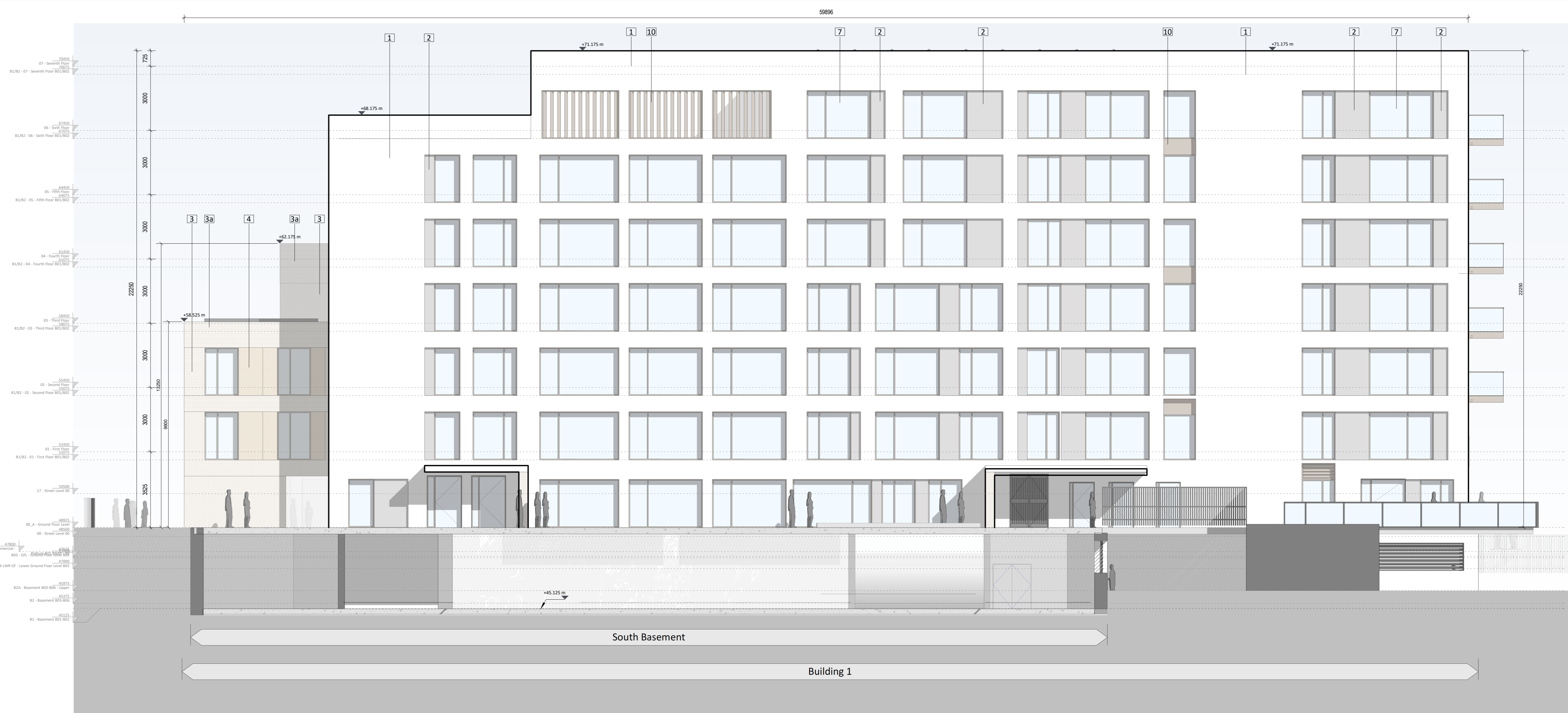
3 Building 01 - SW Elevation 1:100
