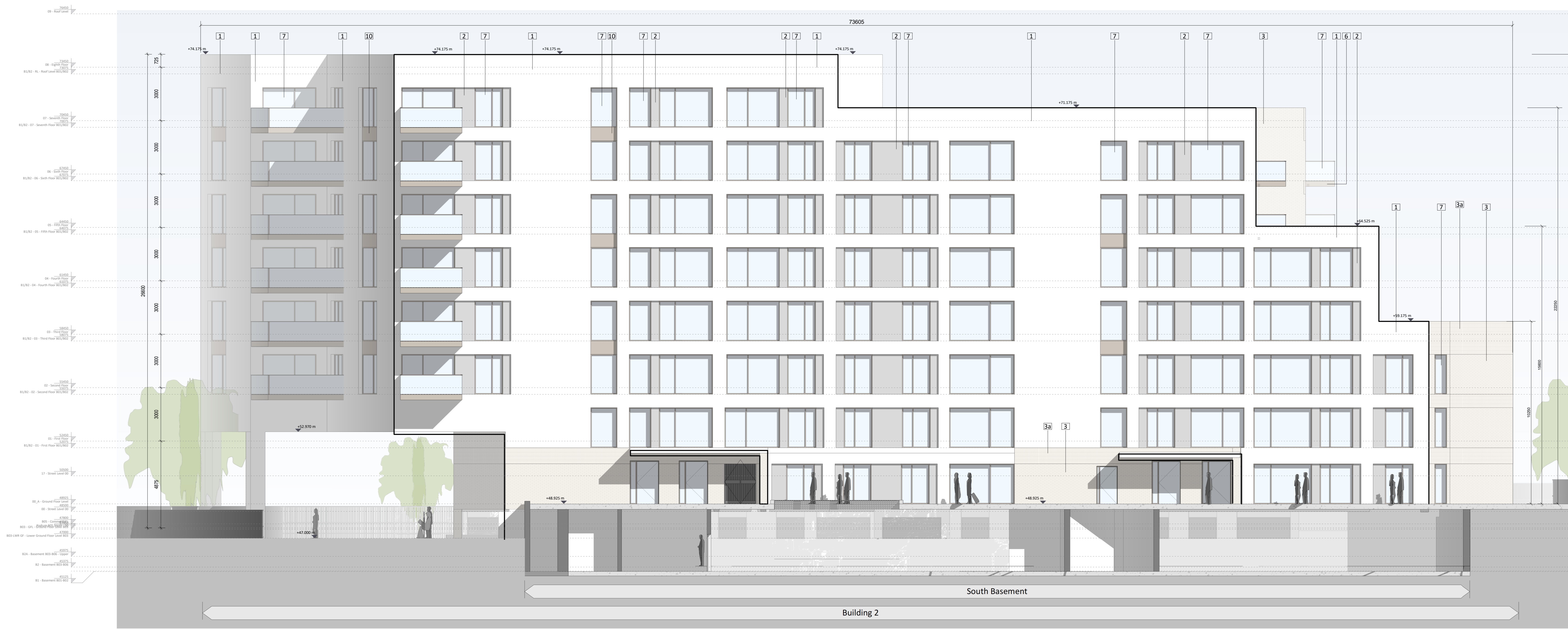
② Building 02 - SW Elevation - Courtyard Elevation 1:100
