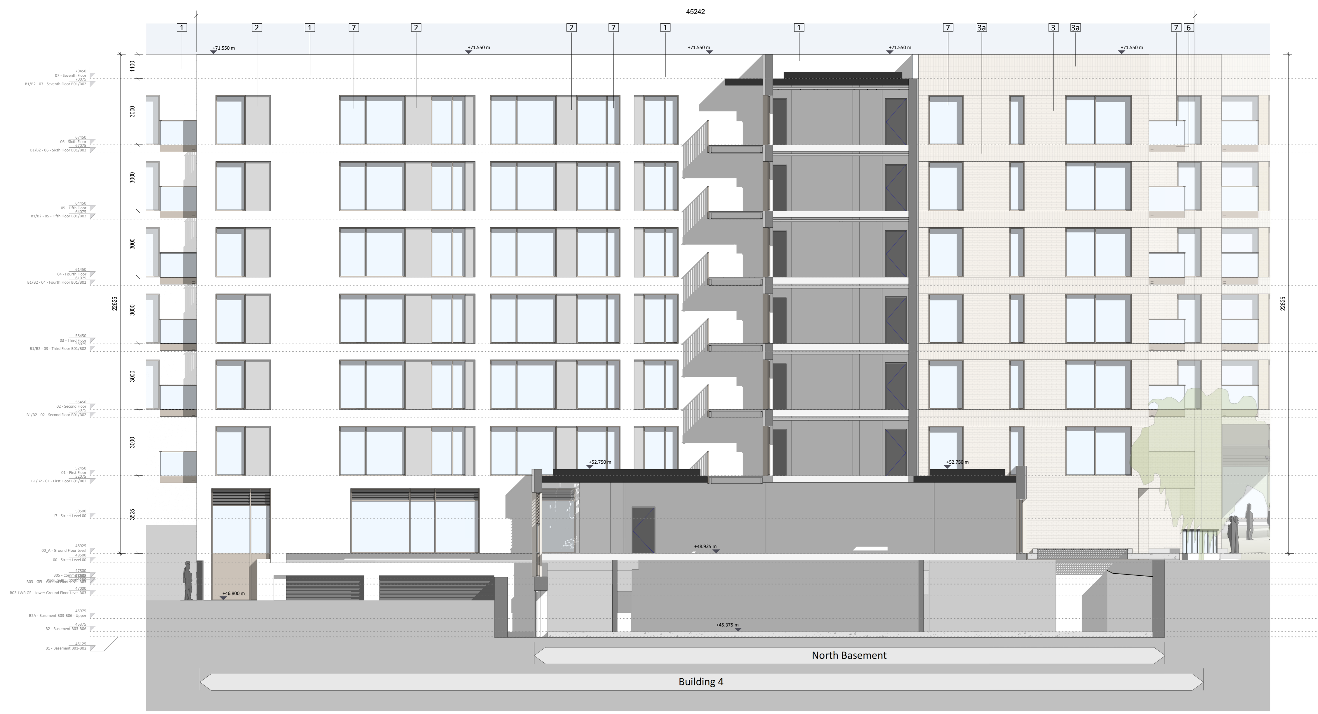
1 Building 04 - NE Elevation - Courtyard Elevation 1:100
