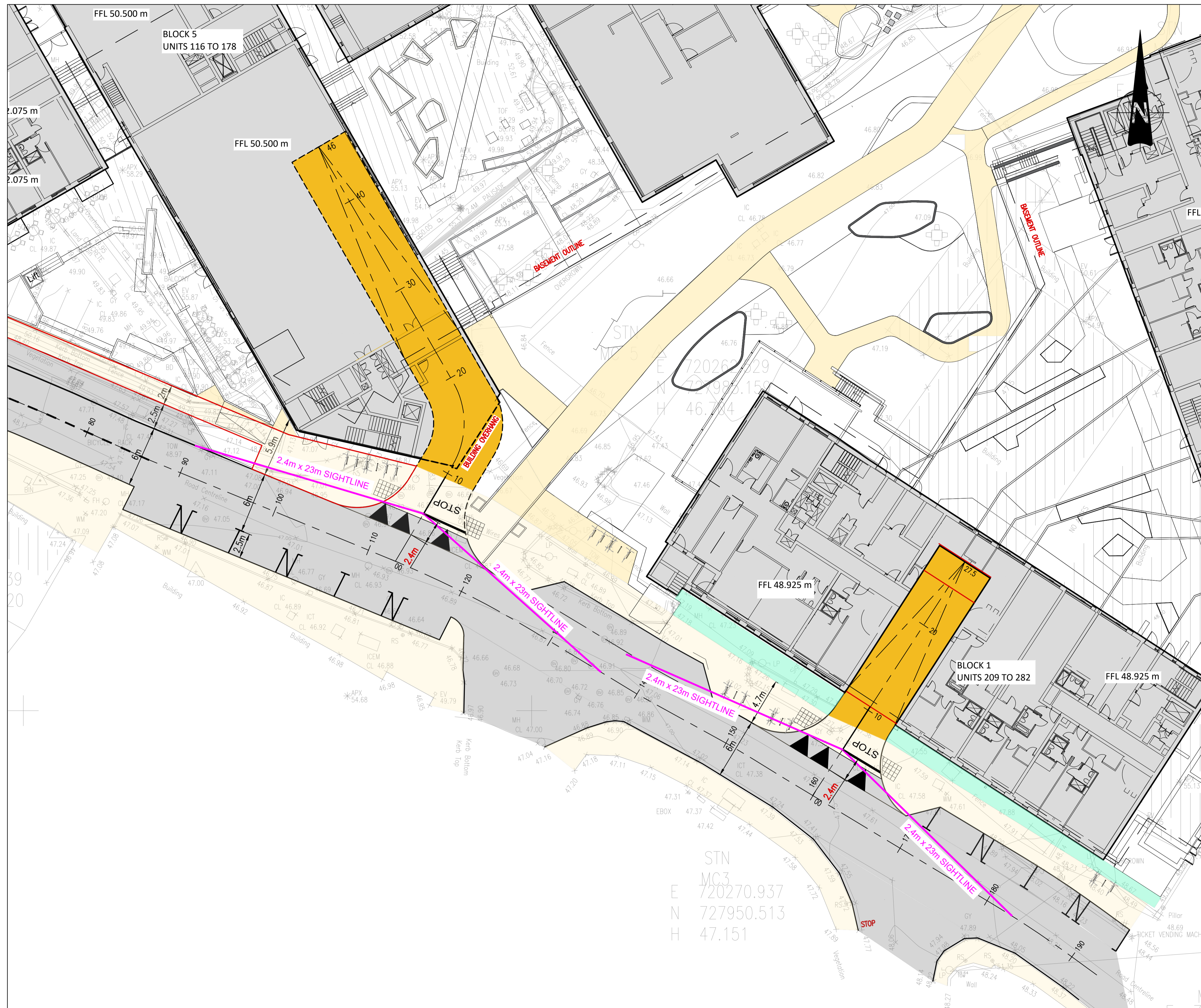
PLAN VIEW PROPOSED SIGHTLINES SCALE 1:200 @A1
